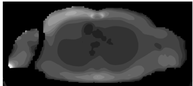
Figure 3. Distribution of tissue temperature in a cross sectional plane across the cerclage, calculated for 3 T MRI. To indicate isothermal lines the number of grey scales was reduced for temperature presentation.
