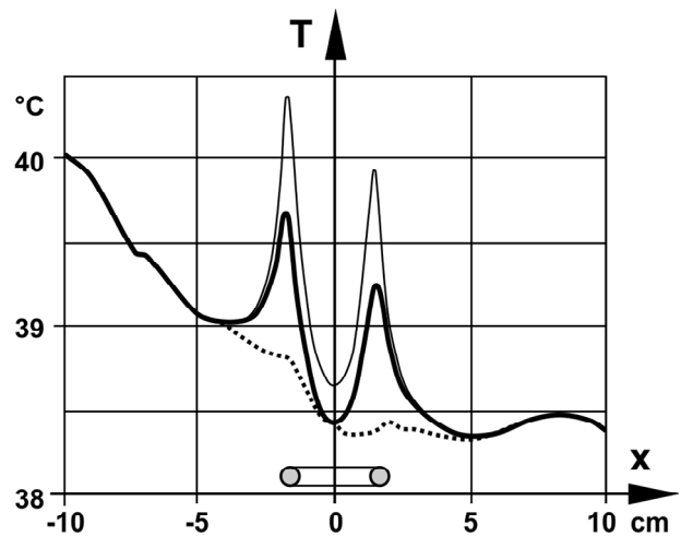
Figure 4. Temperature distribution along the centre line across the cerclage calculated for 1.5 T MRI. Dotted line ... without cerclage, full thick line — cerclage heating based on RF skin effect, full thin line — cerclage heating based on ELF approach with ignored skin effect.
